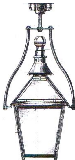
Two arm suspension and ceiling rose With Camberwell
